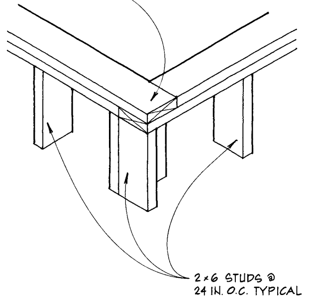
B 2x6 CORNER @ DOUBLE TOP PLATE
