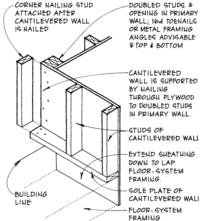
D CANTILEVERED-WALL FRAMING DETAIL @ BASE
