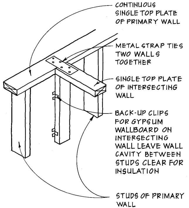
B INTERSECTING 2x WALLS @ TOP PLATE
