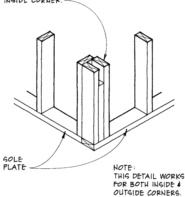
C 2x4 CORNER @ SOLE PLATE
