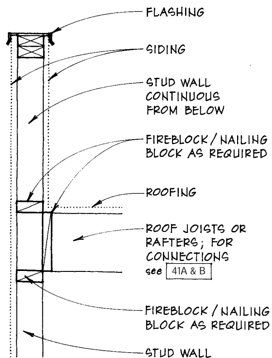
D PARAPET WALL FRAMING ROOF JOISTS SHOWN ⊥ TO WALL
