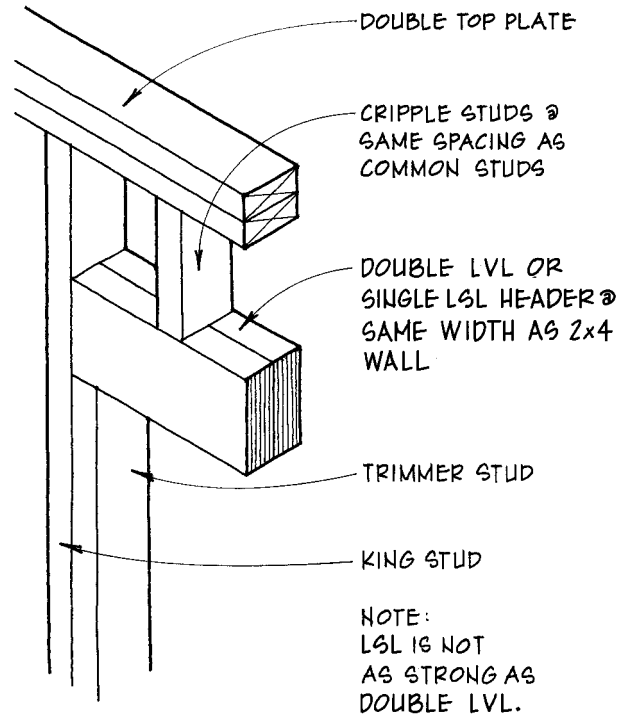
B DOUBLE LVL OR LSL HEADER 2x4 BEARING WALL
