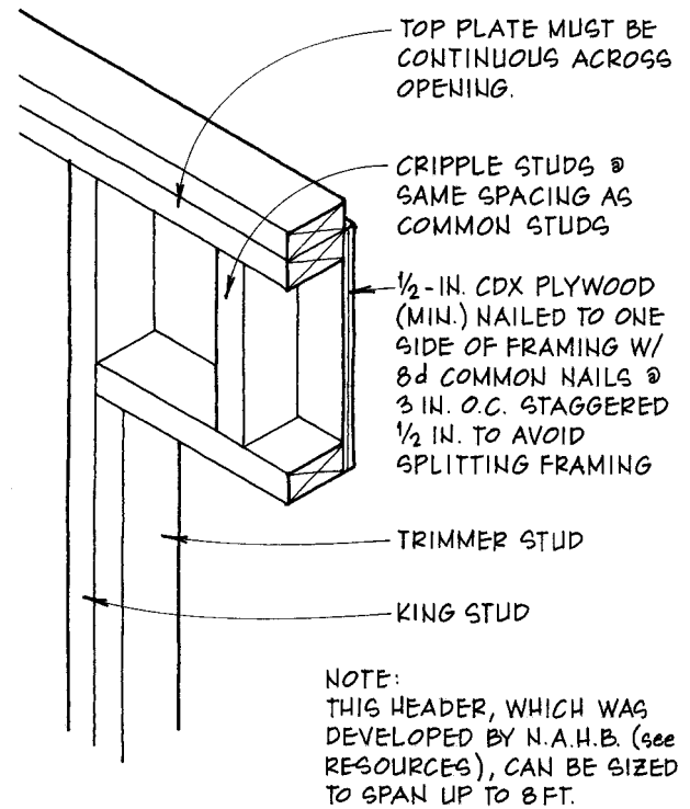
D OPEN-BOX PLYWOOD HEADER 2x4 BEARING WALL
