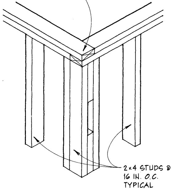
A 2x4 CORNER @ DOUBLE TOP PLATE
