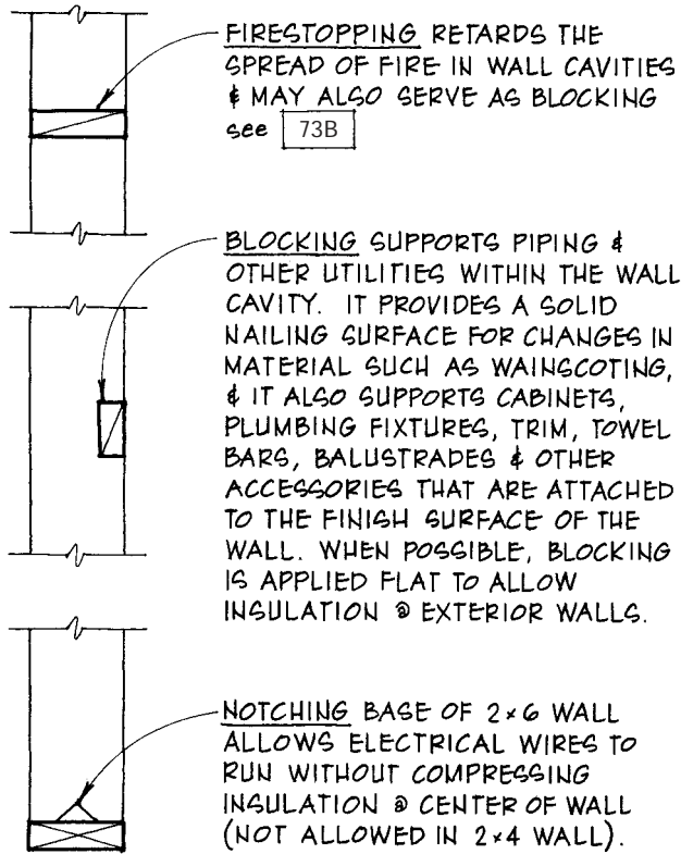
A BLOCKING & NOTCHING
