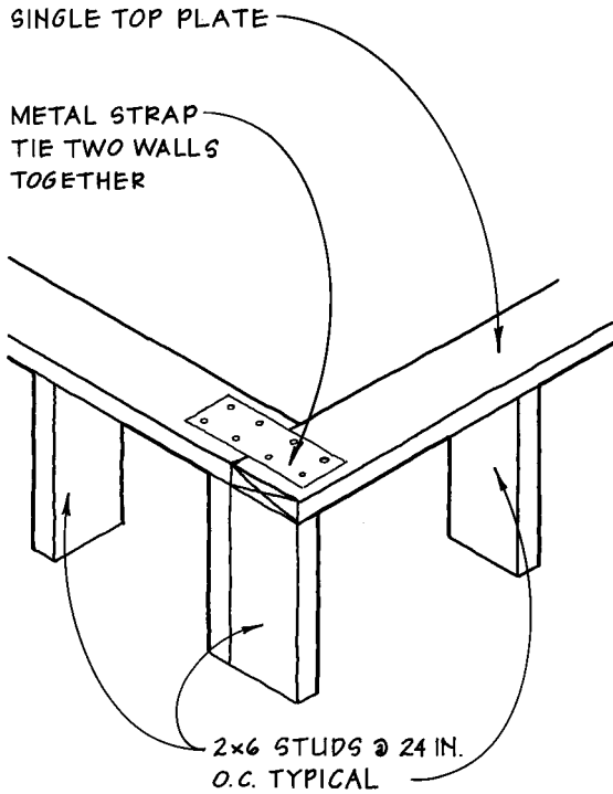
A SUPERINSULATED 2x6 CORNER OUTSIDE CORNER ONLY @ TOP PLATE
