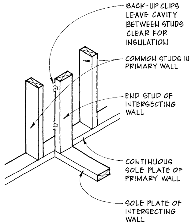
D INTERSECTING 2x WALLS @ SOLE PLATE
