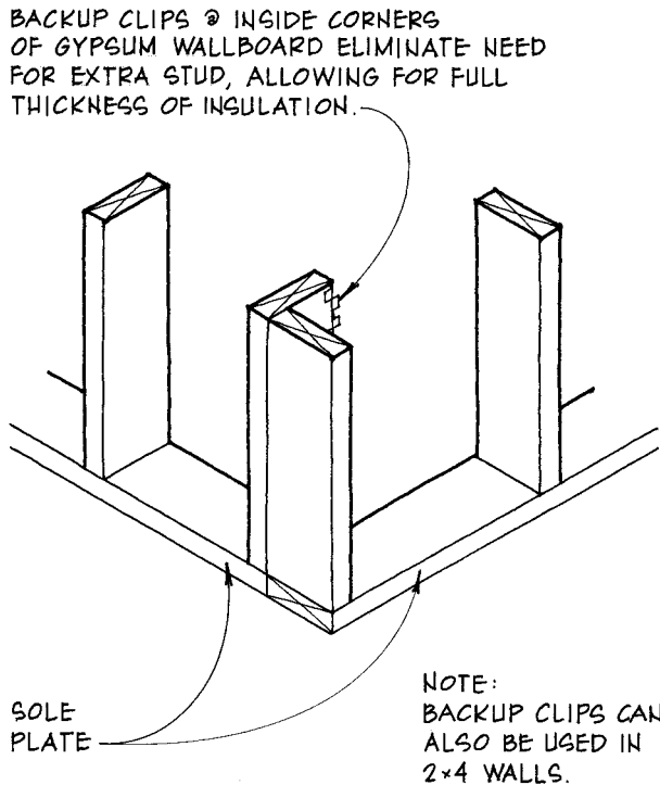
C SUPERINSULATED 2x6 CORNER OUTSIDE CORNER ONLY @ SOLE PLATE
