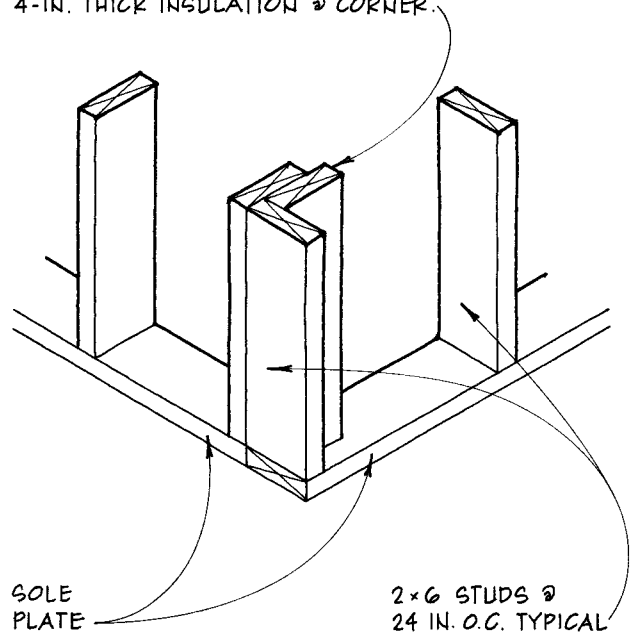
D 2x6 CORNER @ SOLE PLATE
